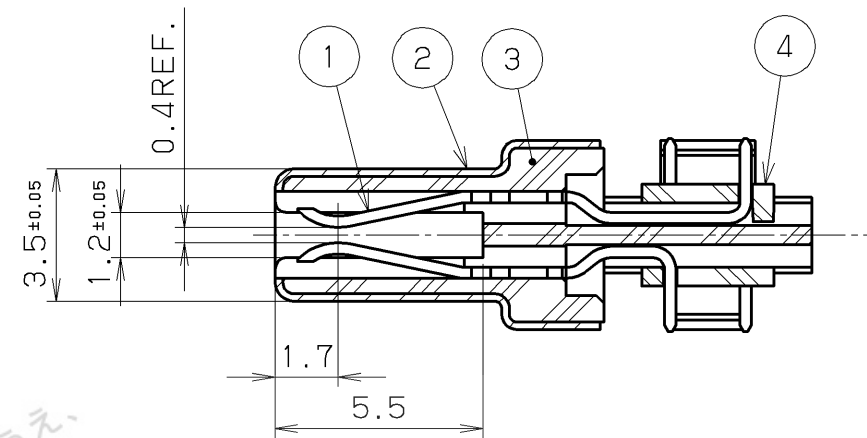
CONTACT DETAIL (5/1)
