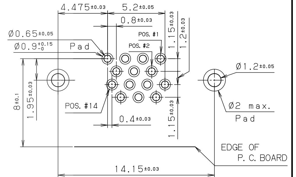
RECOMMENDED P. C. B. LAYOUT (MOUNT SIDE VIEW)
