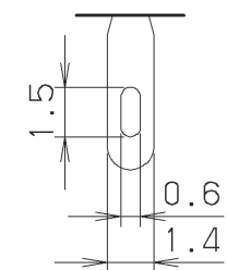
結線部形状 Soldering Part Form
